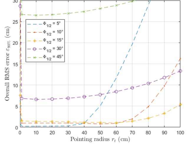
Fig. 2: Evolution of overall RMS error \varepsilon_{90\%} with the pointing radius r_t and the semi-angles at half power \Phi_{1/2} .
