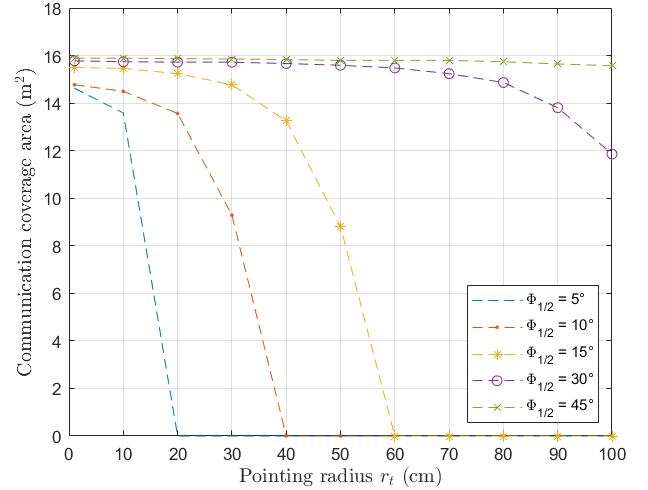
Fig. 4: Evolution of the coverage with the pointing radius r_t and the semi-angle at half power \Phi_{1/2} ( M = 16 ).
