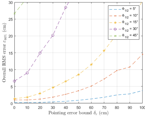
Fig. 3: Evolution of the error \varepsilon_{90\%} with the receiver pointing error bound \delta_r and the semi-angles at half power \Phi_{1/2} .
